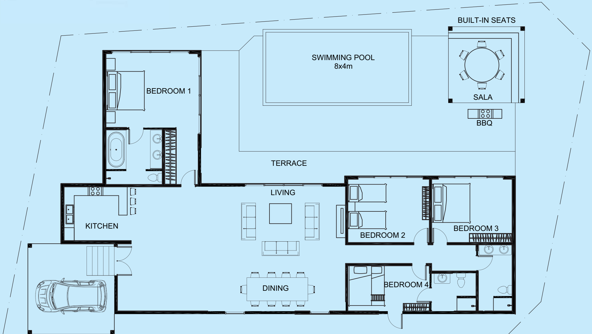
CRYSTAL FLOOR PLAN
